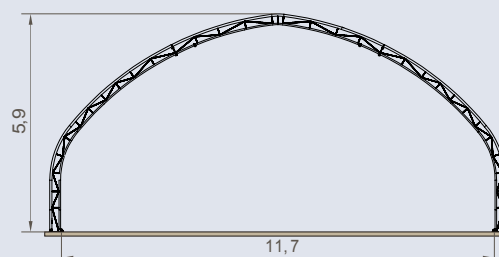
12 m - 2 m moduly
